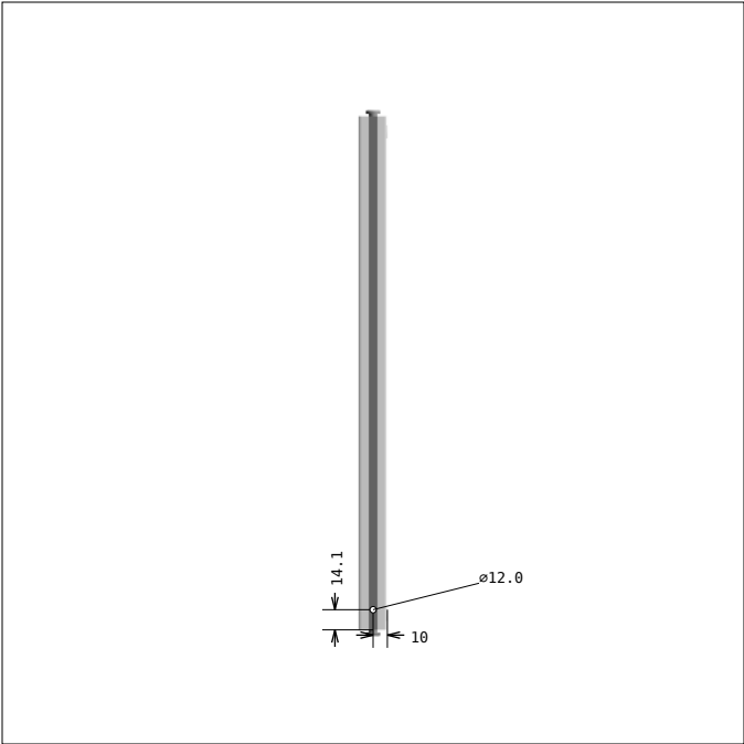
DRAWING 1, Pos 1 SIDE 1, bar length: 360.0 mm
